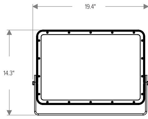
With 3G Mounting Yoke (Factory Installed, Ordered with Luminaire)
