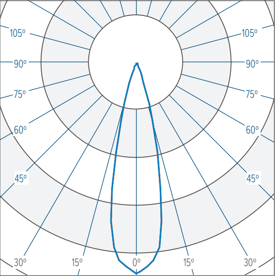
MEDIUM 24° CBCP 8228 @ 1527 Lumens
