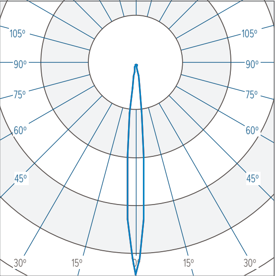
NARROW 13° CBCP 19048 @ 1601 lumens
