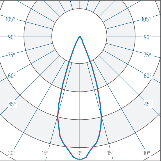
WIDE 45° CBCP 2346 @ 1490 Lumens
