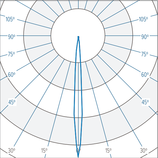
SPOT 10° CBCP 37229 @ 1646 lumens
