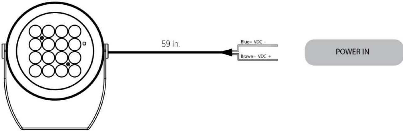
"P" Type Cable (Power In)
