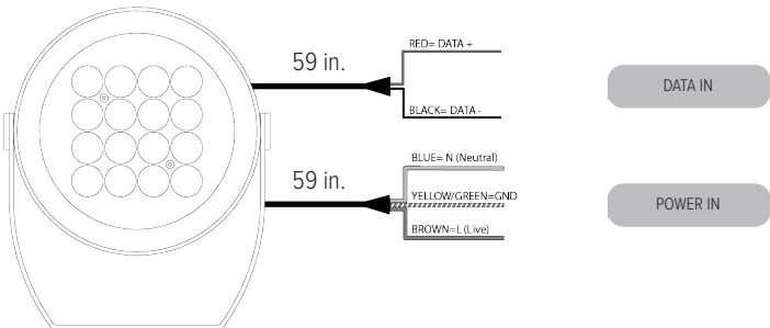
"D" Type Cable (Power in, DALI in, DALI out)
