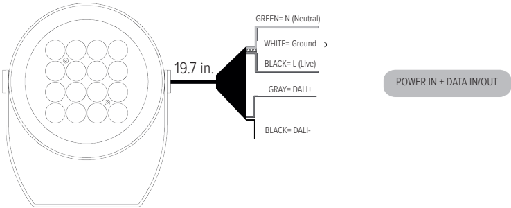
"M" Type Cable (Monocable without connectors for 0-10v Dimming or DALI)
