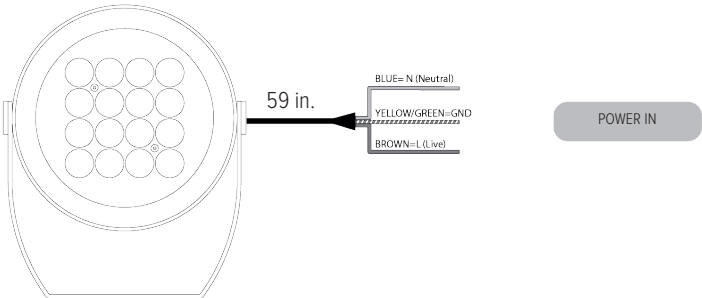
"1" Type Cable (0-10V Dimming)
