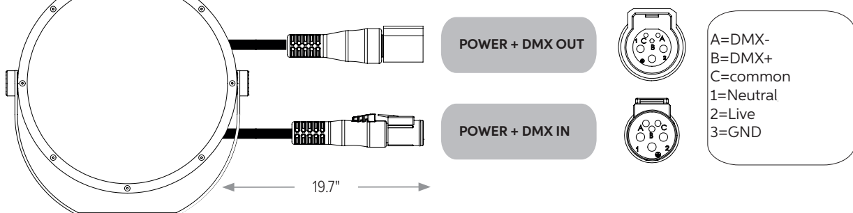
"C" Type Cable (Monocable With Connectors)
